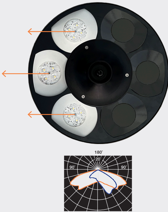
CD Led Evo-3 180°
