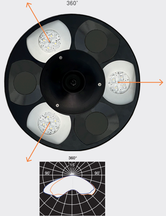
CD Led Evo-3 360°
