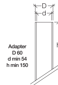
Installation on poles
