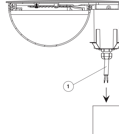
Installation on poles
