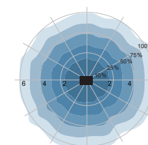
Ceiling mounting pattern Suggested installation height: 2,5-6mt
